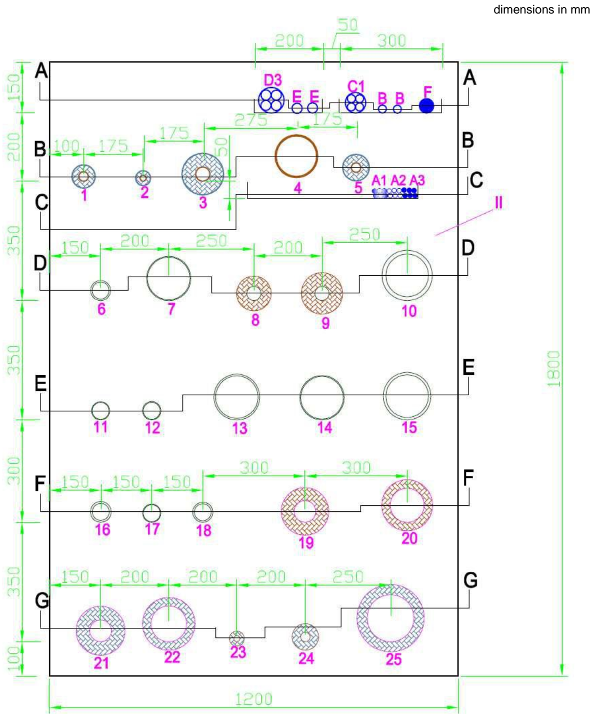
Fig. B1. Minimal distances in mixed penetration seal in wall, made with use of Polylock Elastic
